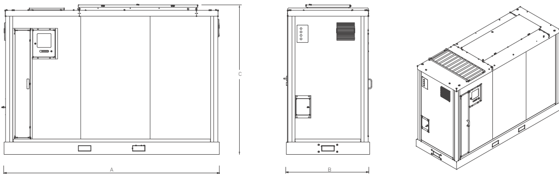
EUROTANK ADBLUE III COMPACT - 3000L - PUERTA DELANTERA
